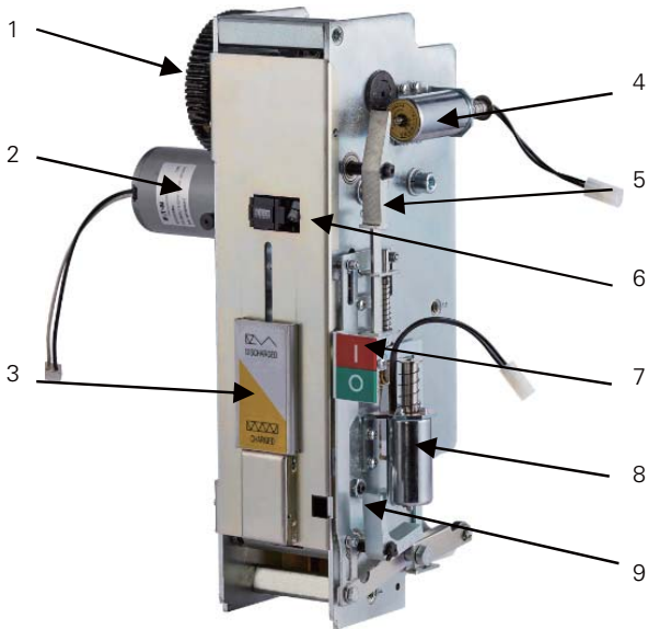
E-Legend Mechanism
