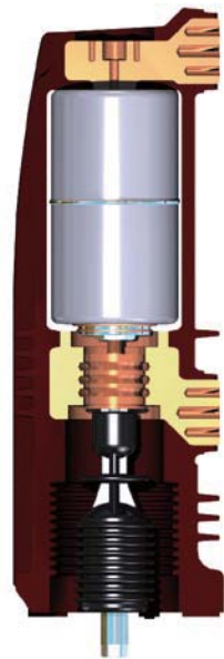
Encapsulated pole unit (EPU)
