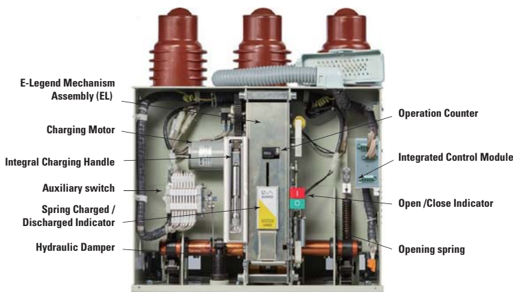
Internal view of W-VACi Circuit Breaker Element
